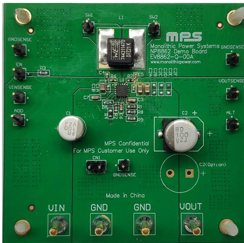
Figure 2: EV8862-Q-00A Evaluation Board
