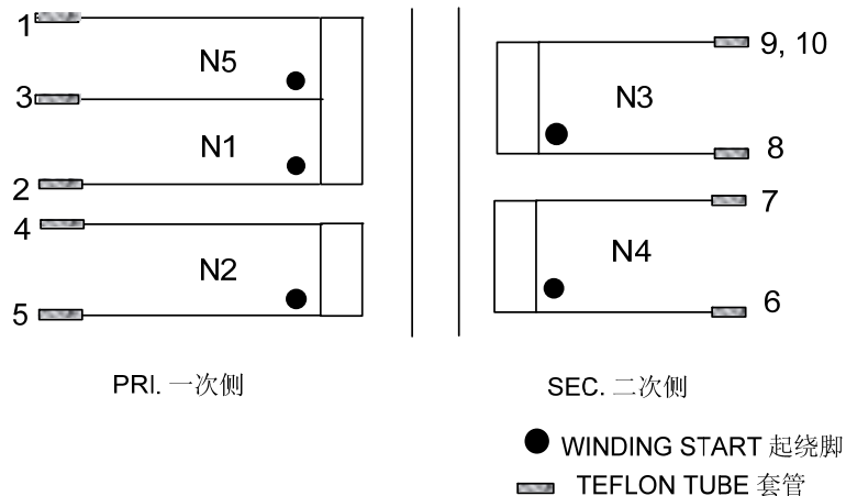
Pin Definition of Bobbin
