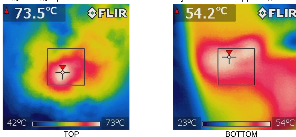
Vin=85Vac, Thermal Performance
