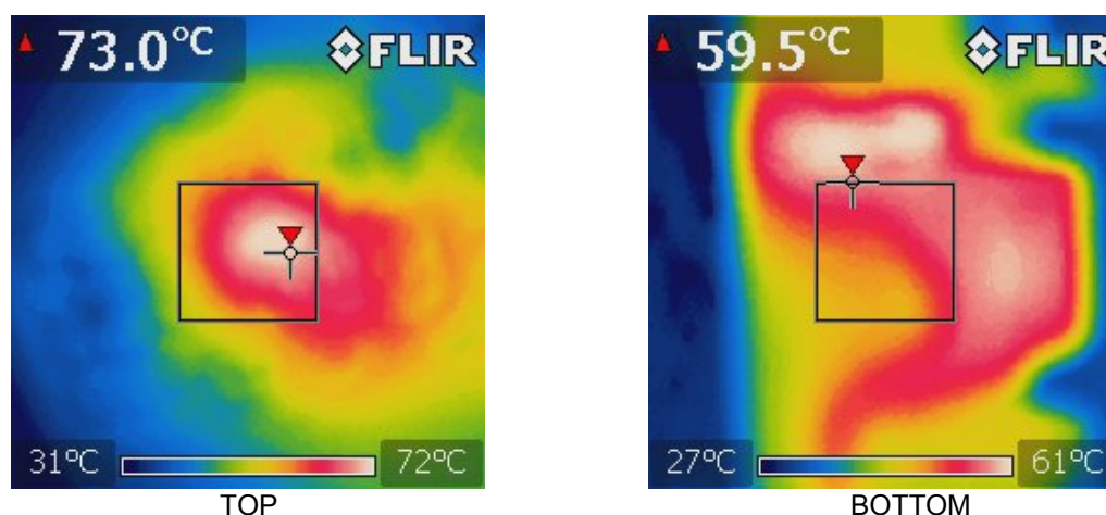
Vin=265Vac, Thermal Performance
