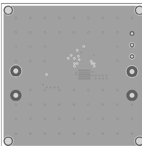
Figure 5: Bottom Layer
