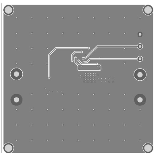
Figure 4: Mid-Layer 2
