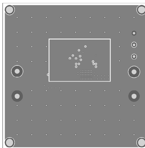
Figure 3: Mid-Layer 1
