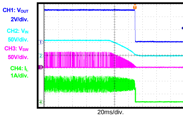
Power Off I_{OUT}=1A
