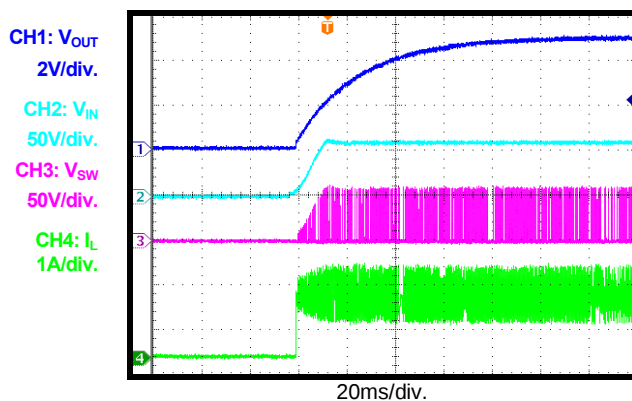
Power On I_{OUT}=1A
