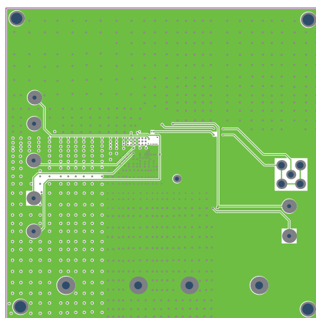
Figure 4—Inner Layer 2
