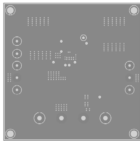
Figure 4—Inner2 Layer
