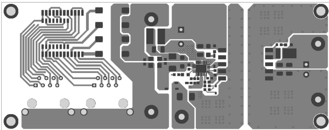
Figure 2: Top Layer
