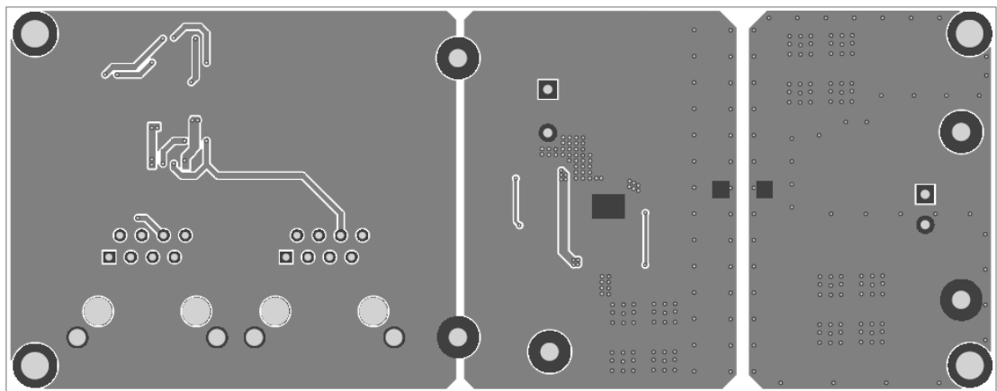
Figure 3: Bottom Layer
