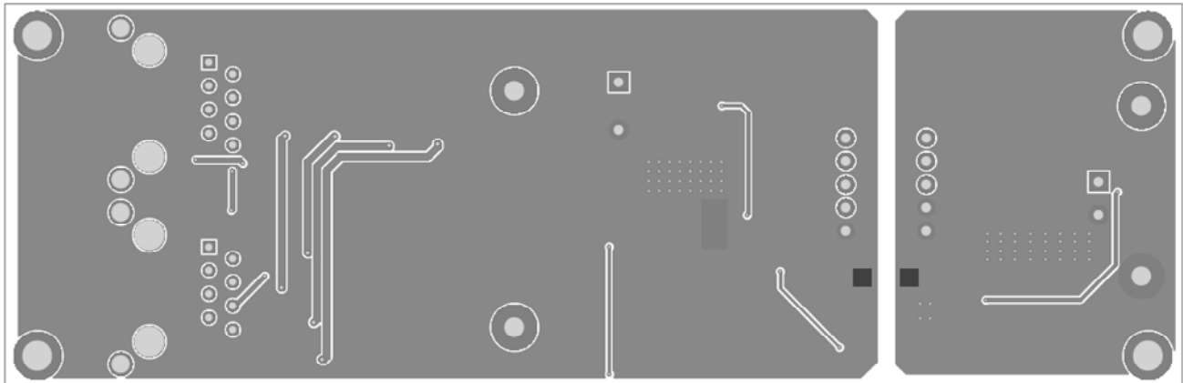
Figure 3: Bottom Layer
