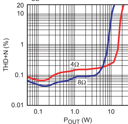
THD+N vs Output Power V_{DD} = 24V, f = 1KHz
