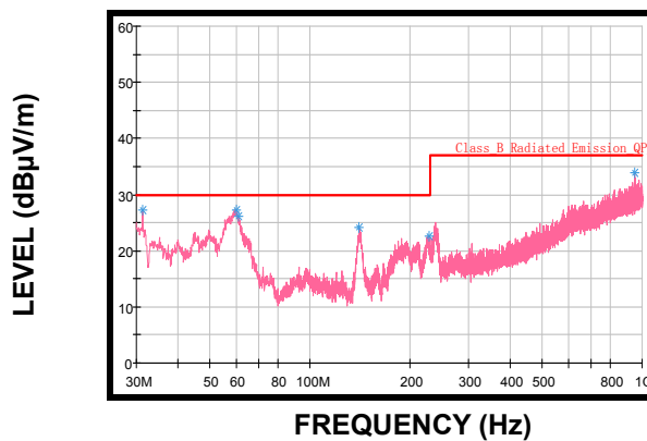
Radiated Emission Results
