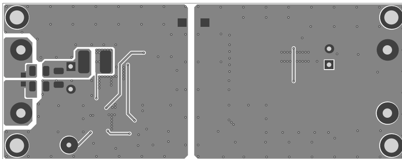
Figure 4: Bottom Layer
