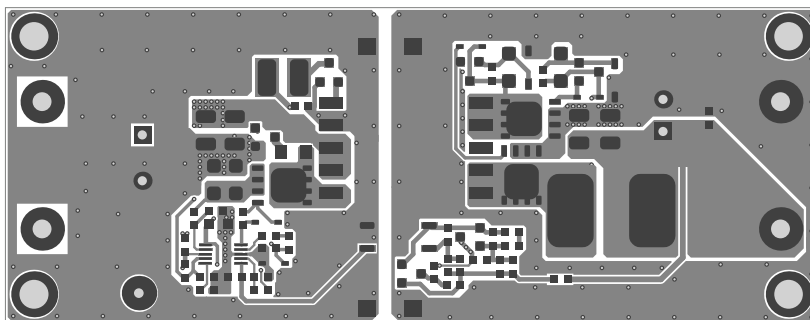
Figure 2: Top Layer
