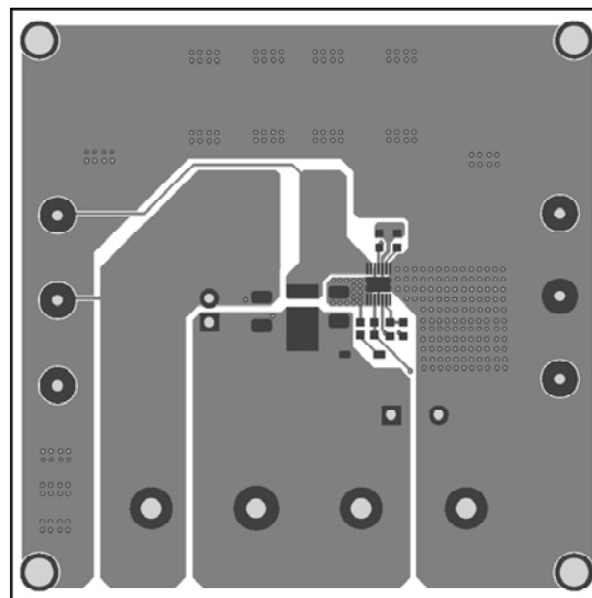
Figure 2: Top Layer
