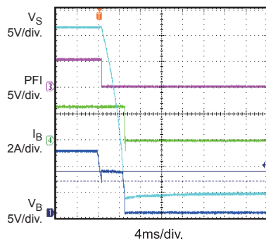
V_{STRG} Release
