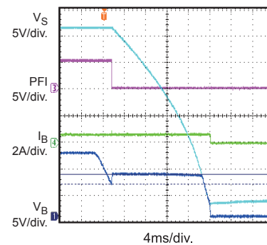
V_{STRG} Release
