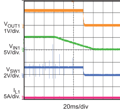
VIN Power Down without Load (CH1)
