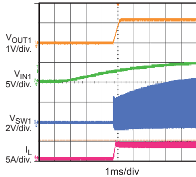
VIN Power Up with 3.5A Load (CH1)
