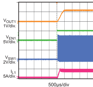
EN On with 3.5A Load (CH1)
