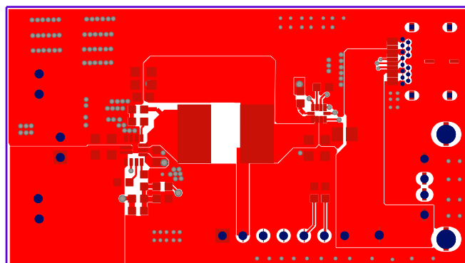
Figure 2: Top Layer
