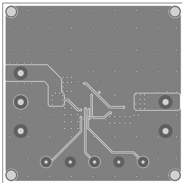
Figure 3—Inner2 Layer
