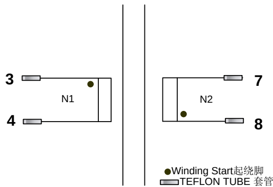
Electrical Diagram
