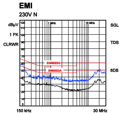
Figure 6—230 VAC, 50 Hz, maximum load, N line, EN55022 limits
