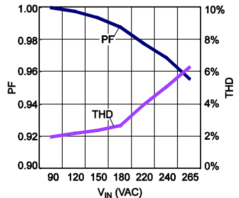
PF & THD
