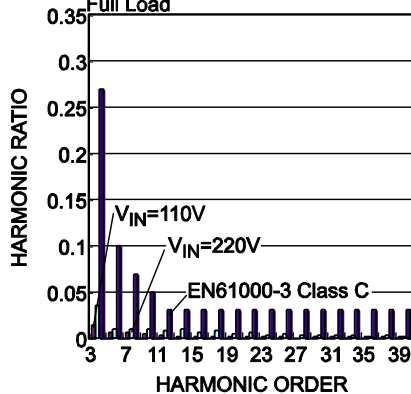
Harmonic
