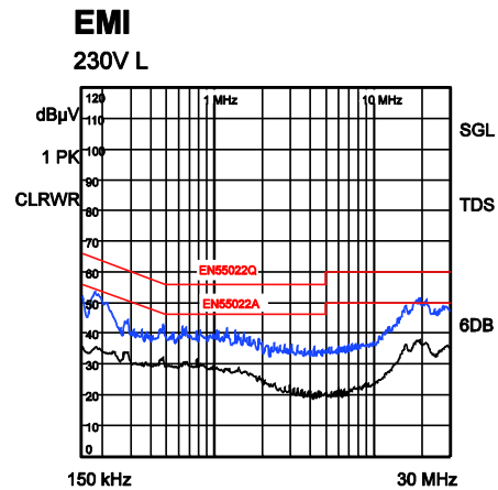
Figure 5—230 VAC, 50 Hz, maximum load, L line, EN55022 limits
