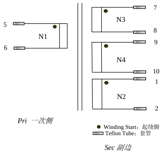
Pin Definition of Bobbin
