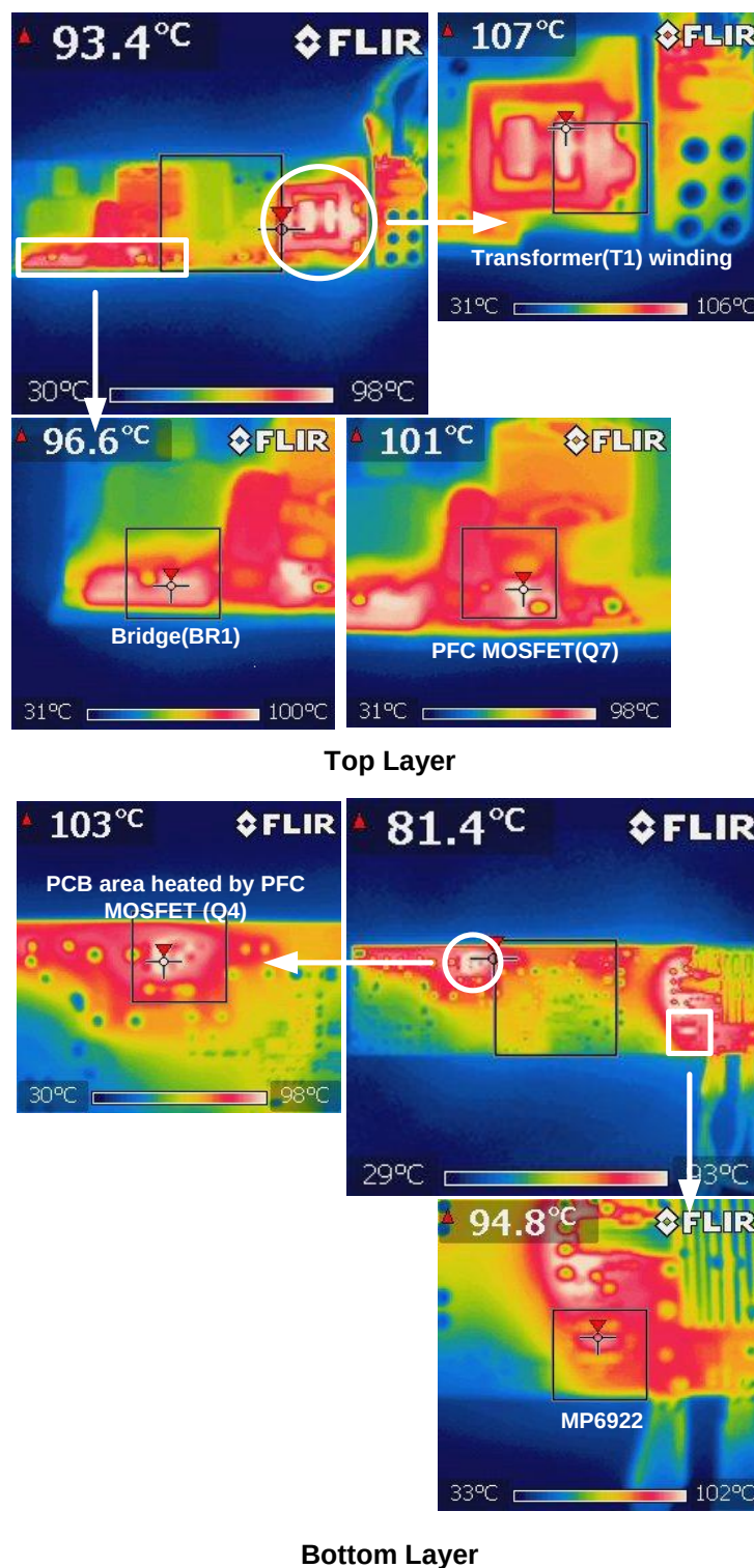
Figure 7—Temperature chamber test
