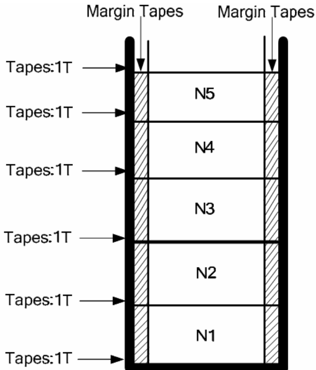
Winding Diagram
