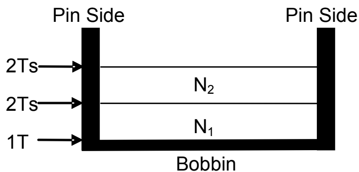
Figure 5—Winding Diagram
