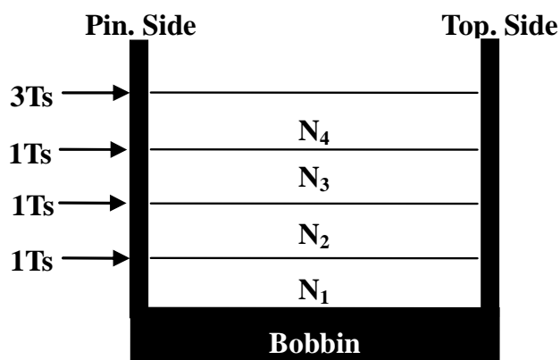
Figure 5—Winding Diagram
