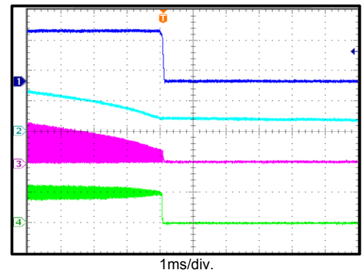
Shutdown through Input Voltage I_{OUT} = 2A
