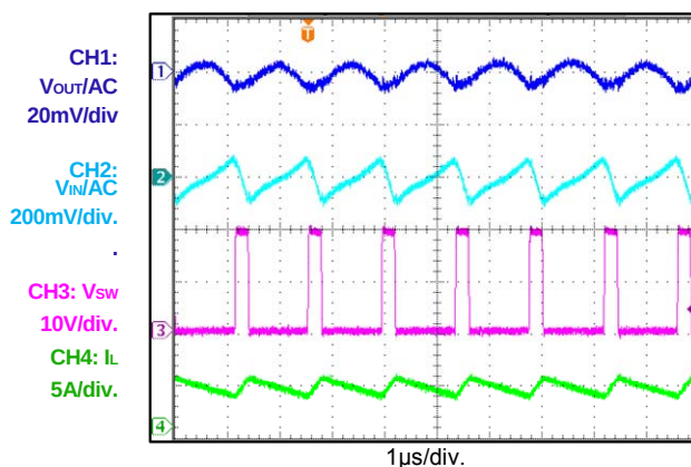
Input/Output Ripple I_{OUT}=4A
