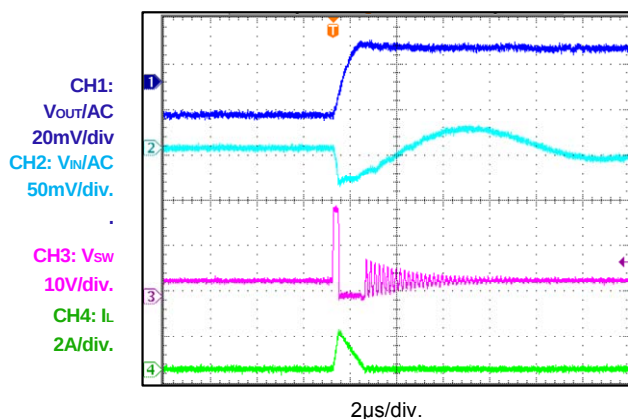
Input/Output Ripple I_{OUT}=0A
