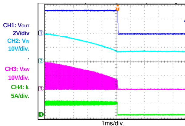
Shutdown through Input Voltage I_{OUT}=4A
