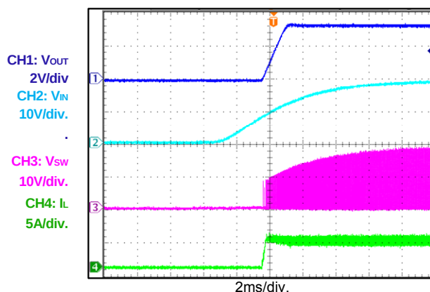
Startup through Input Voltage I_{OUT}=4A
