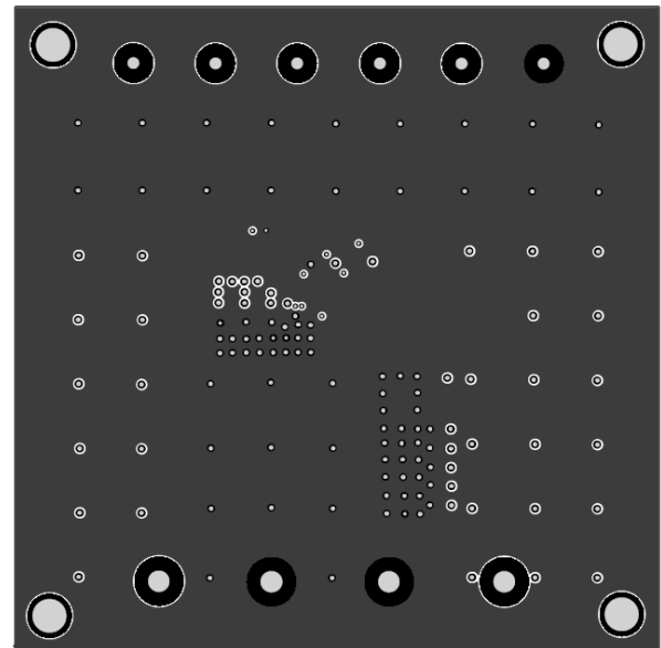
Figure 2: Inner Layer 1
