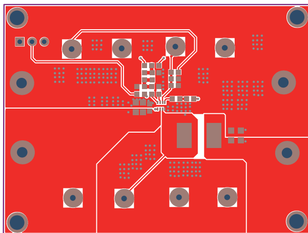
Figure 2: Top layer
