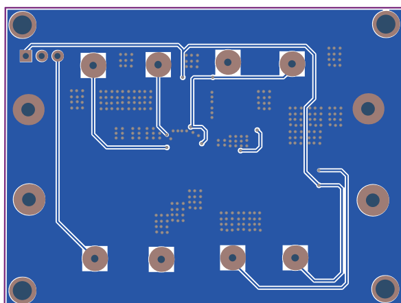
Figure 3: Bottom layer
