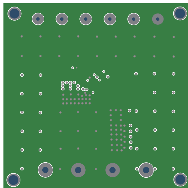
Figure 2—Inner Layer 1
