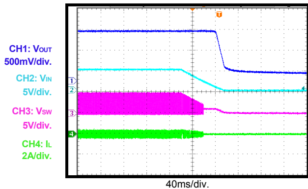
V_{IN} Shutdown
