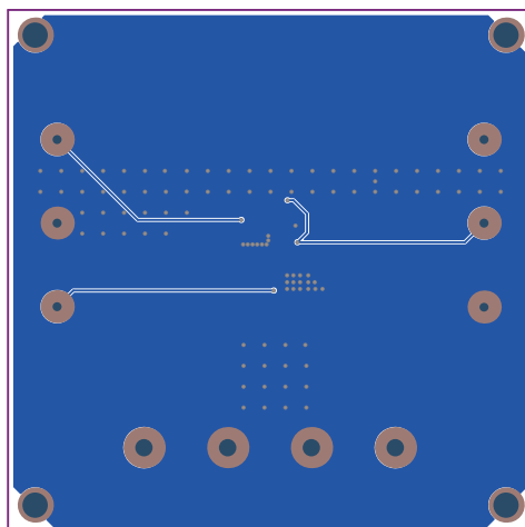
Figure 4: Bottom Layer
