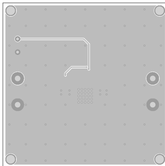
Figure 2: Bottom Layer
