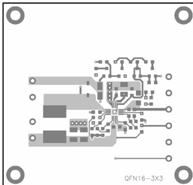
Figure 2: Top Layer
