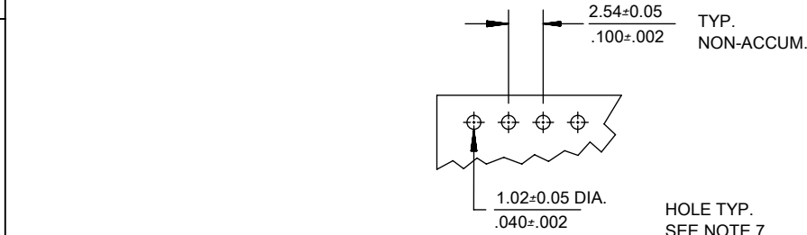
TYP. HOLE PATTERN FOR 1.57/.062 THK. PCB
