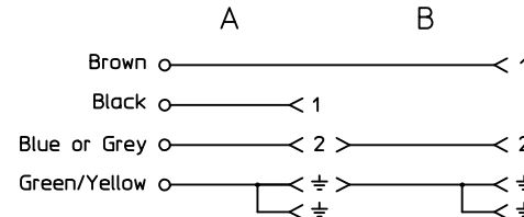
ELECTRICAL DIAGRAM E653XXXXXX1X000
