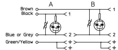
ELECTRICAL DIAGRAM E653XXXXXX1XS0X
