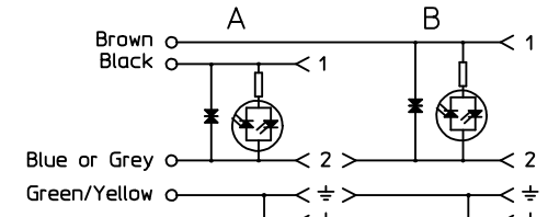
ELECTRICAL DIAGRAM E653XXXXXX1XS0X
