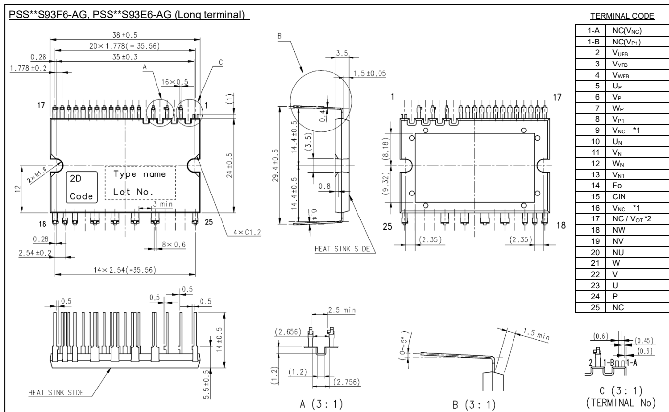
Fig. 10 Package Outlines
