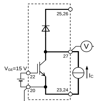
Brake IGBT
