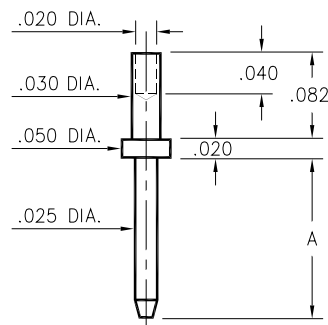
3120-X-00-XX-00-00-08-0 Swage mount in .034 mounting hole
