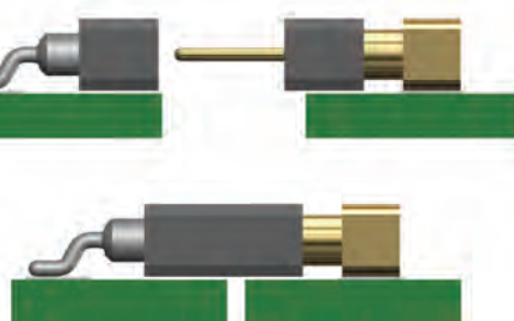
Z-Bend Style SIP Socket HSMT (2,54 Grid)
