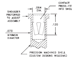
#34 CONTACT FOR .032"-.046" DIAMETER PINS ( \delta = .010 ) 4-FINGER, GROUP E (See page 248)
