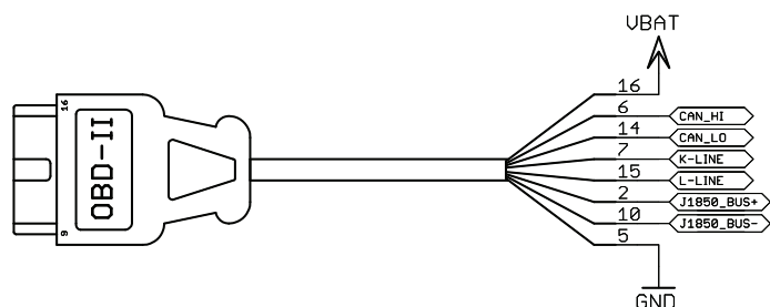
Figure 3 – OBD Connections
