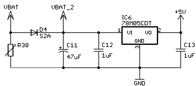
Figure 7 – Power Supplies
