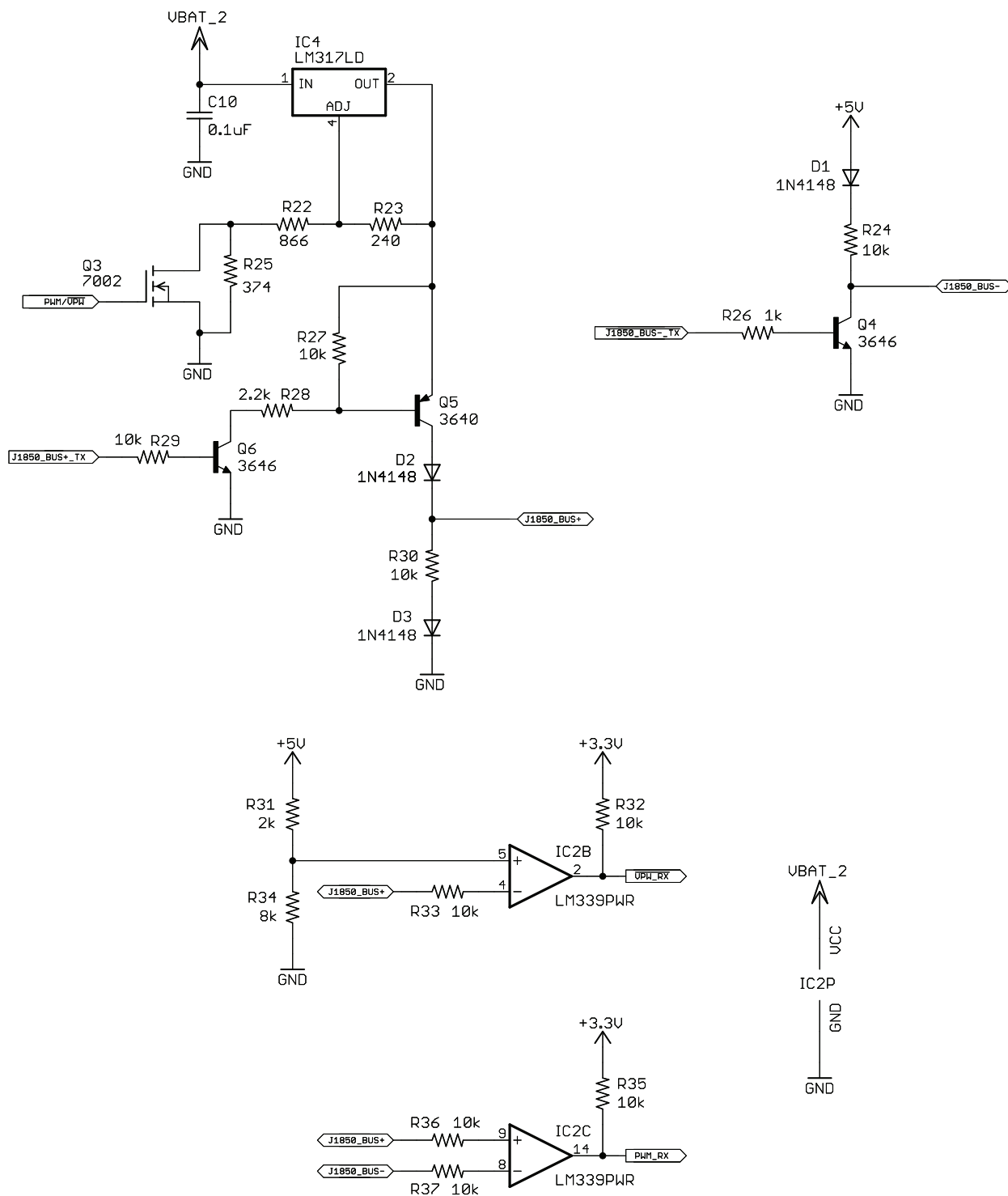
Figure 6 – J1850 Transceiver
