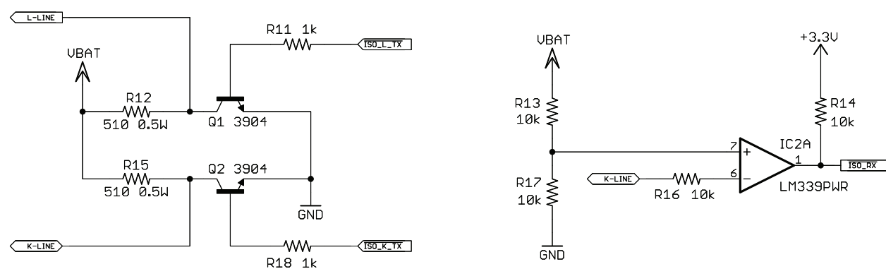
Figure 4 – ISO Transceiver
