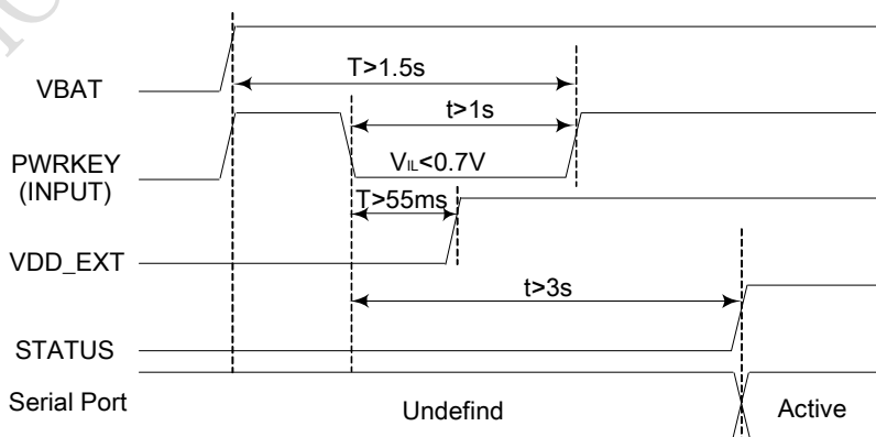
Figure 12: Timing of power on module
