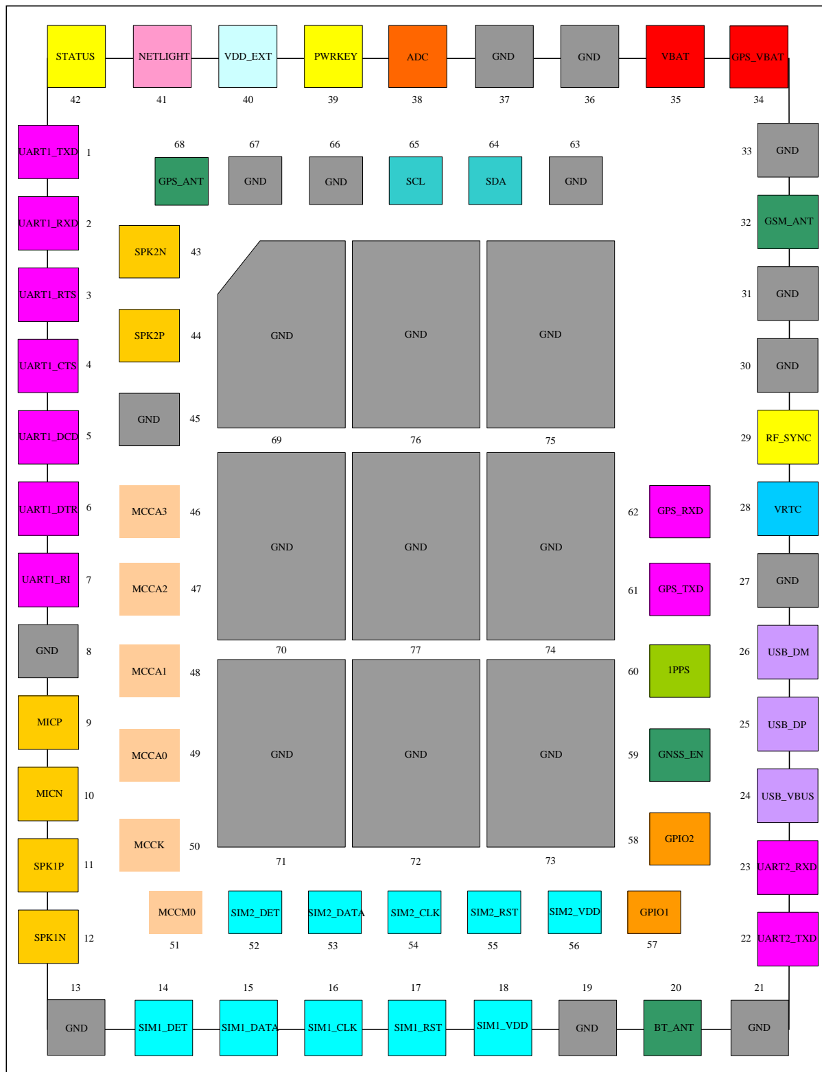
Figure 41: PIN assignment
