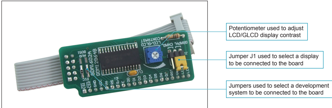
Figure 1: Serial LCD/GLCD Adapter additional board
