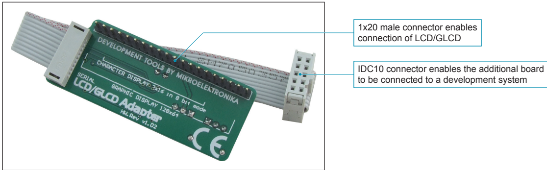
Figure 2: Back of the Serial LCD/GLCD Adapter additional board
