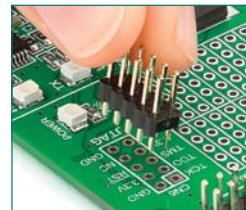
Figure 3-11: placing 10 pin header
