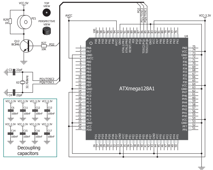
Figure 8-2: Piezo buzzer connection schematics
