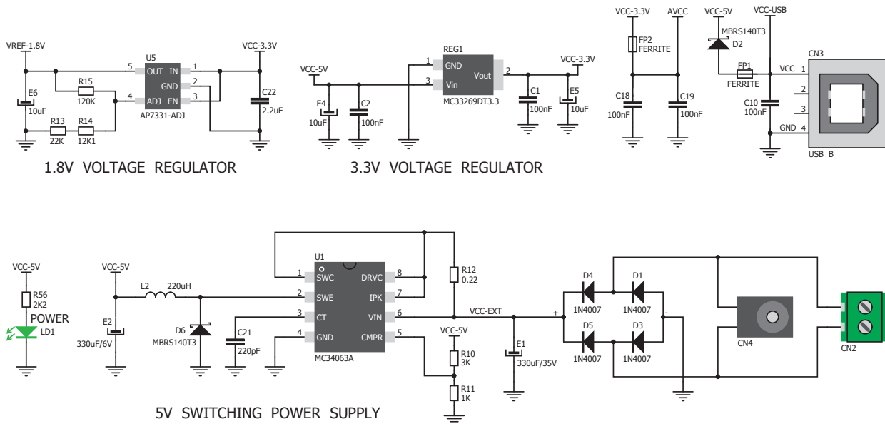
Figure 1-4: Power supply schematics
