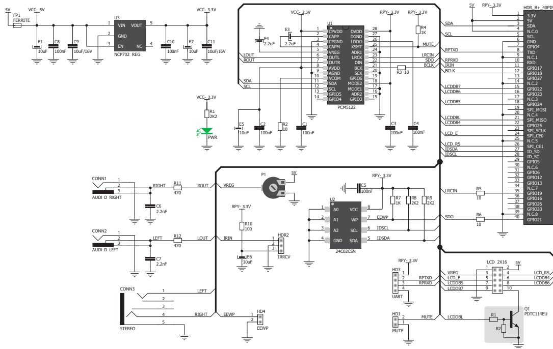
Figure 2: RaspberryPlay4 schematic
