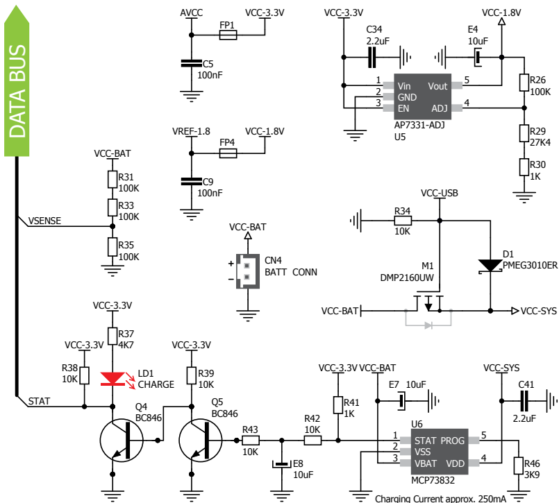
Figure 1-3: Power supply schematics
