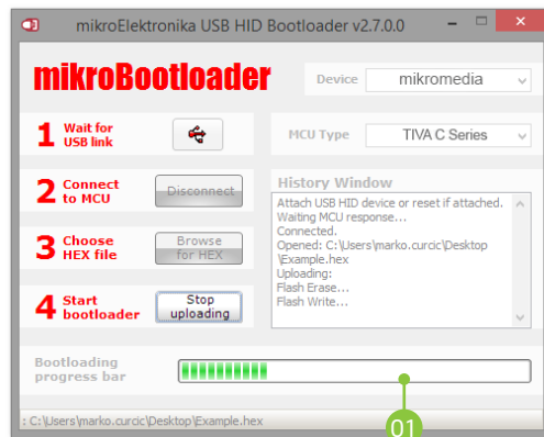
Figure 3-6: Progress bar
