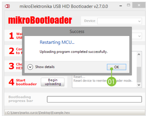
Figure 3-7: Restarting MCU
