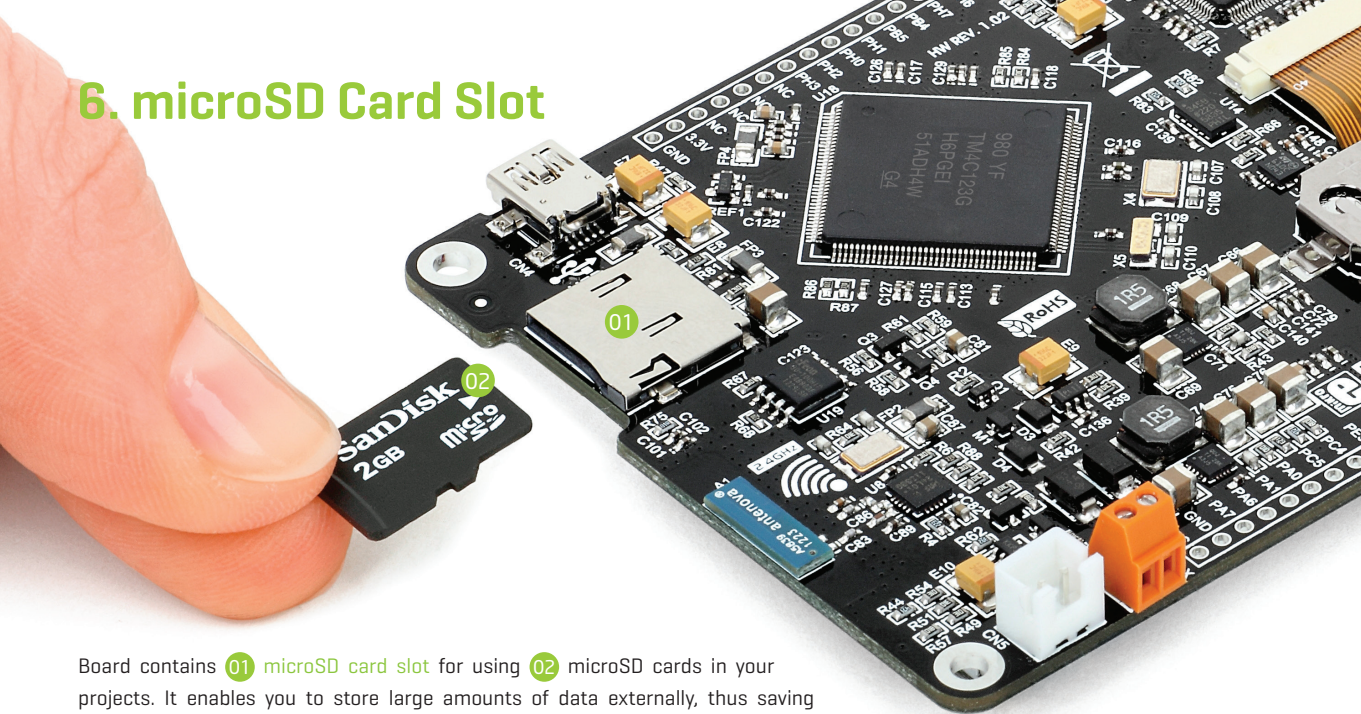
Figure 6-1: microSD card slot
