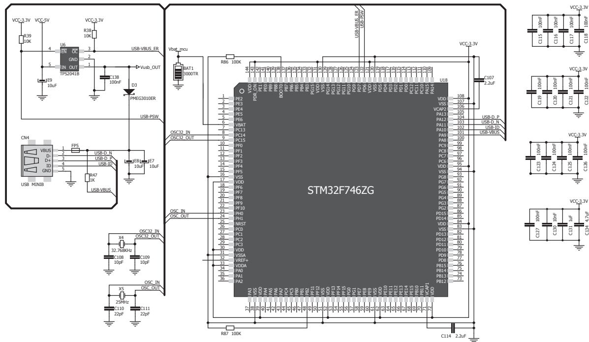
Figure 10-2: USB HOST module connection schematic
