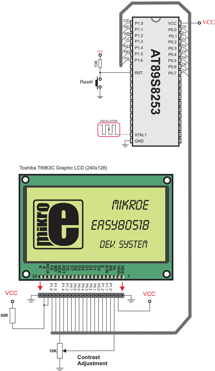
6.17. T6963C GLCD HW connection
