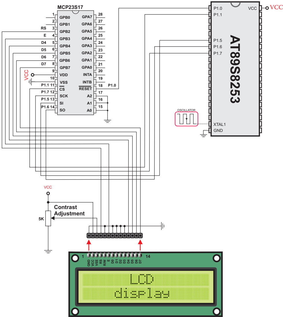
6.14.SPI LCD HW connection
