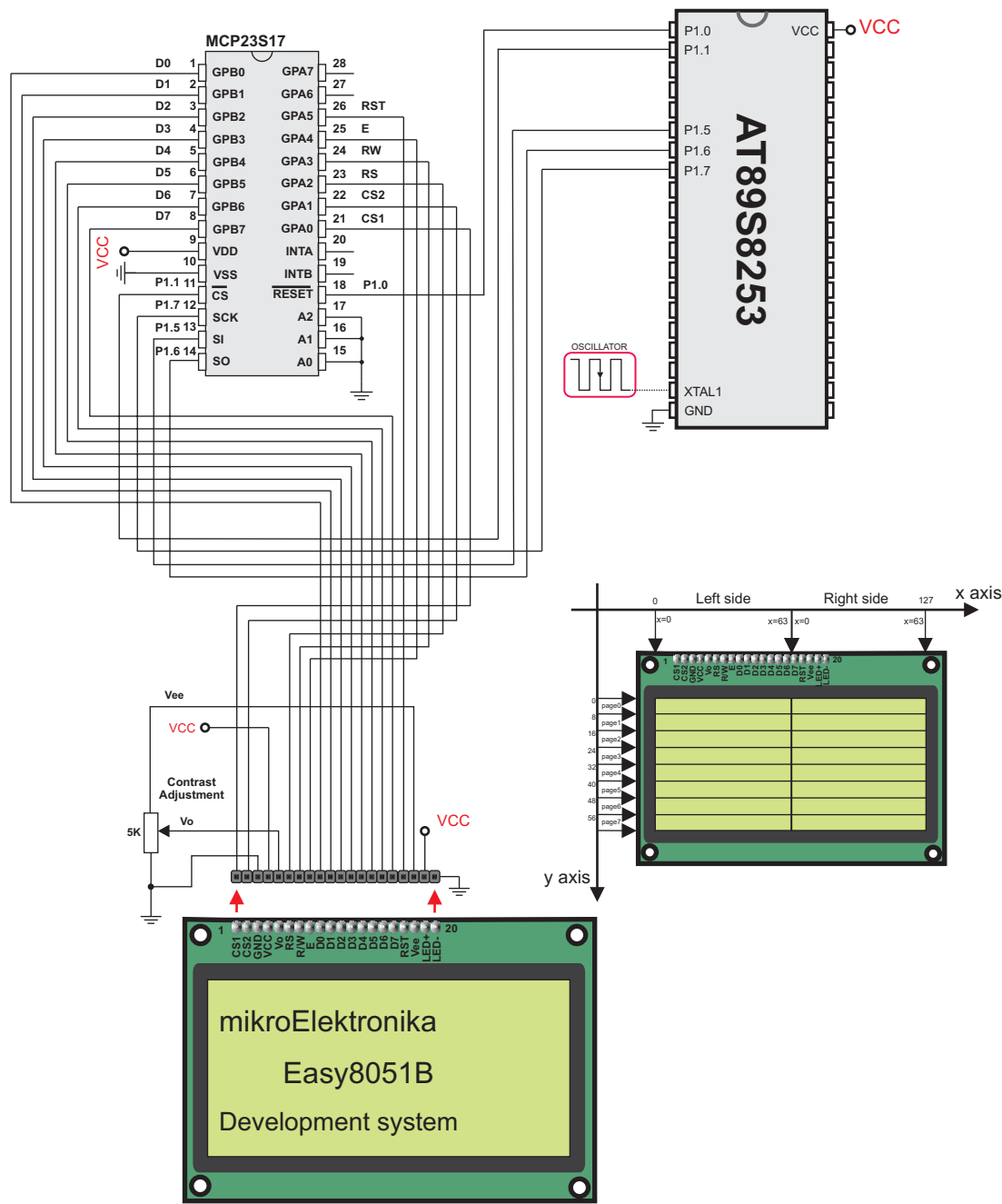
6.13. SPI GLCD HW connection
