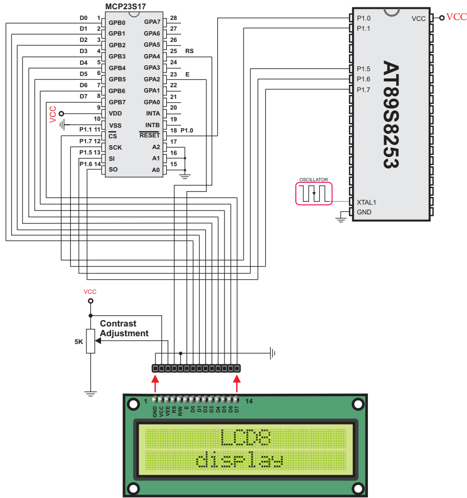
6.15. SPI LCD8 HW connection
