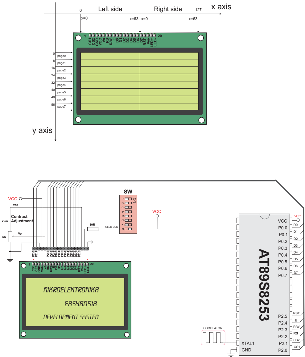
6.2. GLCD HW connection
