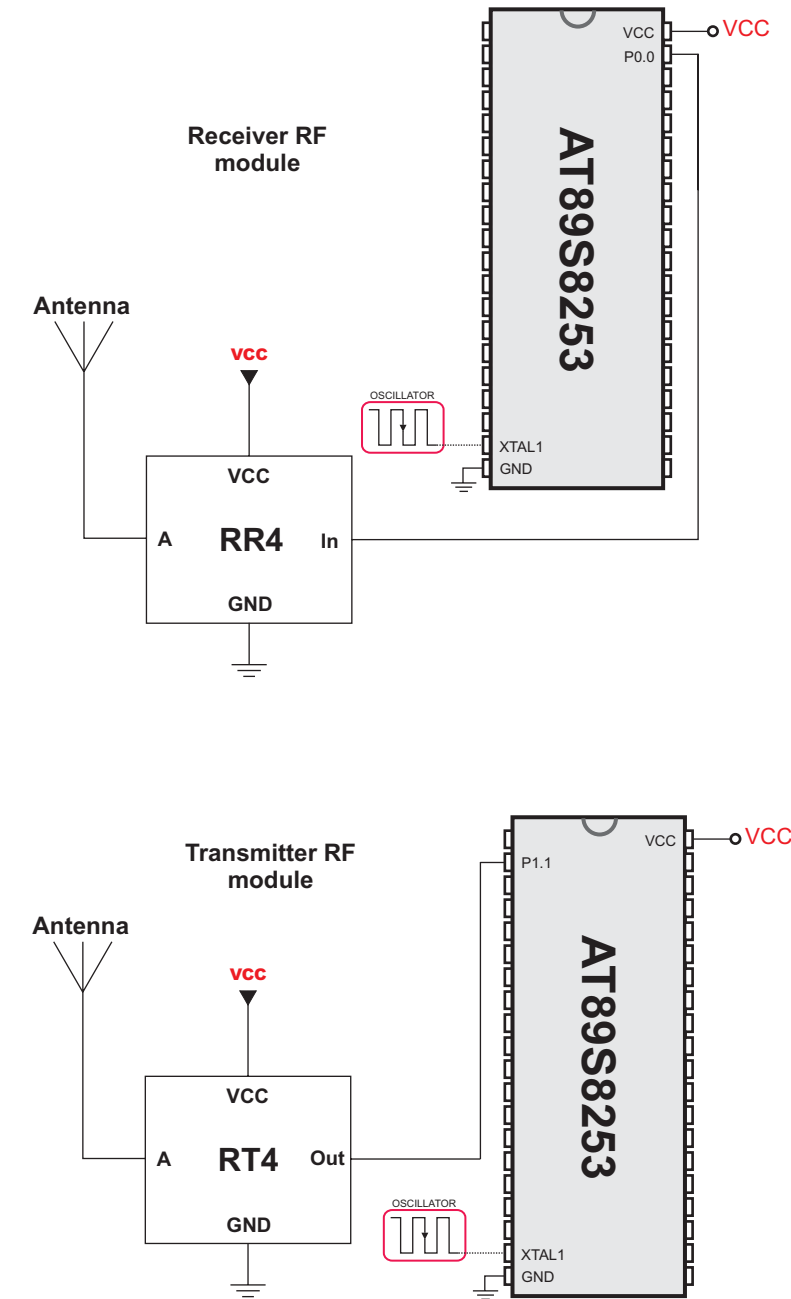
6.6. Simple Receiver connection
