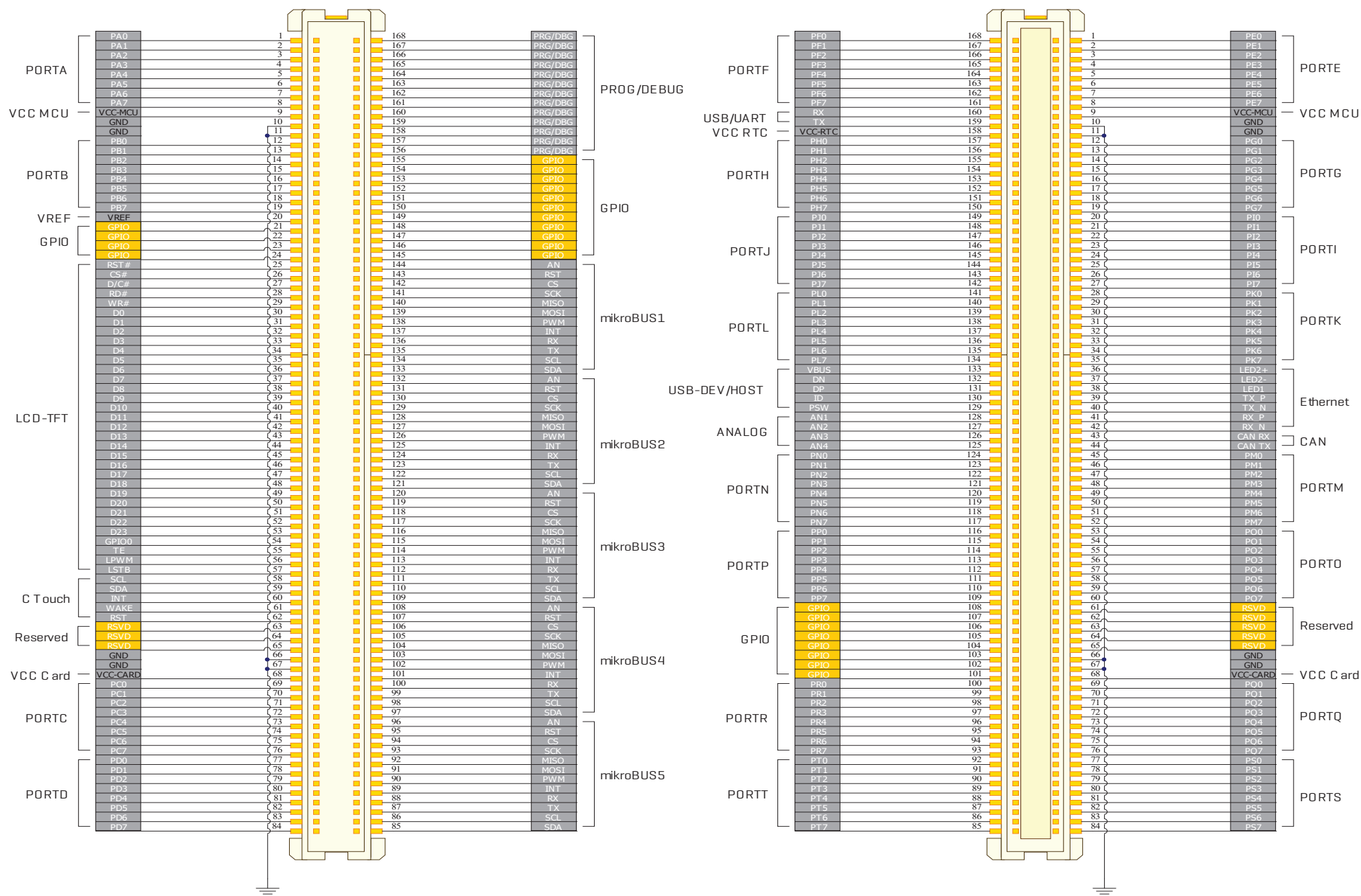
MCU Card Connectors Schematic
