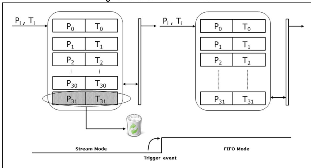
Figure 10. Stream-to-FIFO mode
