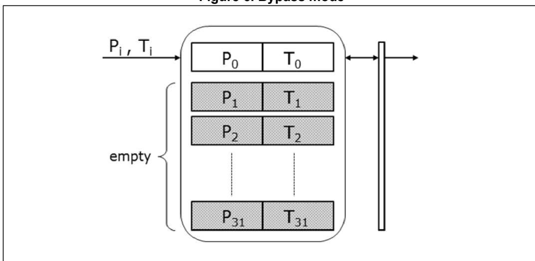
Figure 6. Bypass mode
