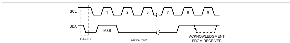
Figure 8. Acknowledge on the I 2 C BUS
