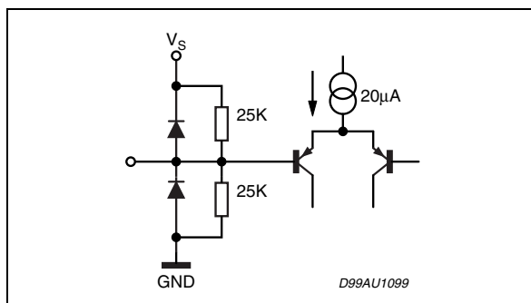
Figure 18. PIN: CREF
