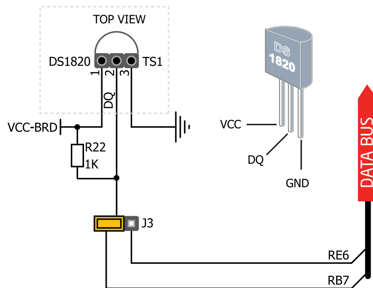
Figure 16-5: DS1820 connected to RB7 pin
