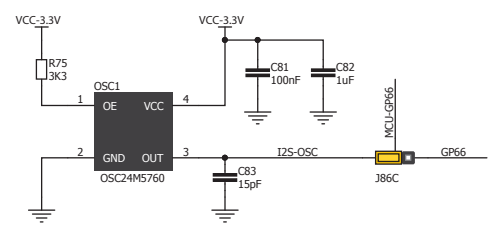
Figure 13-1: Schematic of I 2 S module
