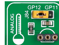
Figure 24-3: LM35 socket
