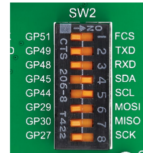
Figure 25-2: Turn on switches SW2.4 and SW2.5 to connect EEPROM lines to MCU
