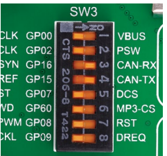
Figure 12-2: enabling CAN communication
