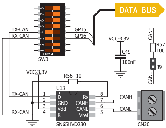
Figure 12-1: CAN connection schematic
