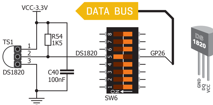
Figure 23-2: DS1820 socket
