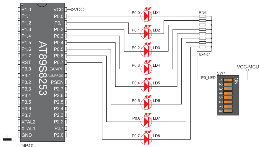
Figure 9-2: LED diode and port PORT0 connection schematic
