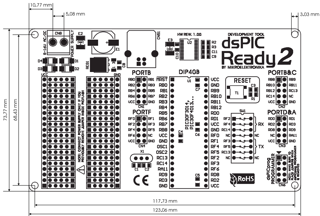
Figure 4: Dimensions of the dsPIC Ready2 additional board
